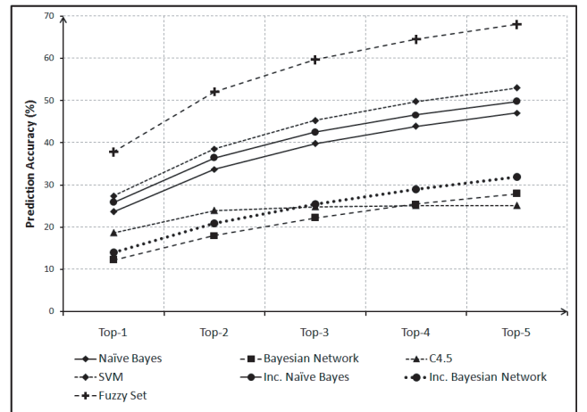
Figure 3: Prediction Accuracy Comparison
